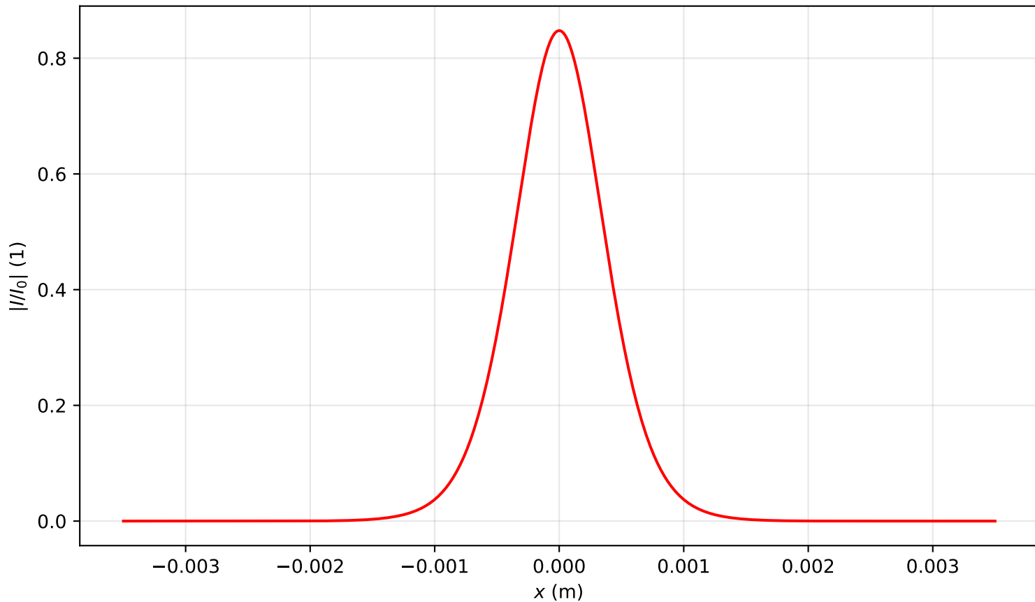
Intensity profile I(x, y = 0, z = 1.911)/I_0 , P_{in}=0.5P_{cr} , artificial time
